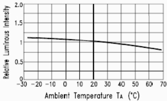
Fig.5 Luminous Intensity vs. Ambient Temperature T_A ( ^{\circ}\text{C} )
